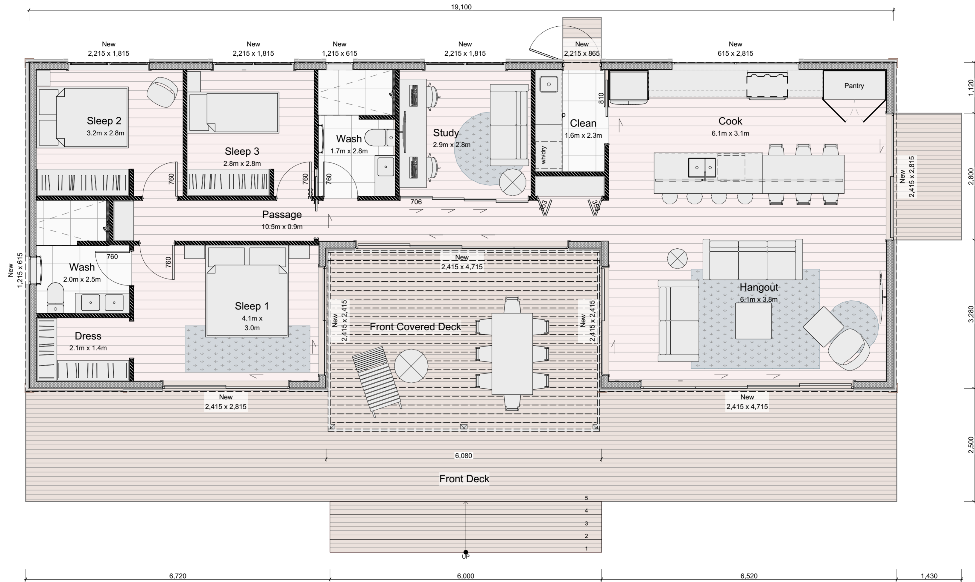
The Retreat 120m2 scale 1:50
