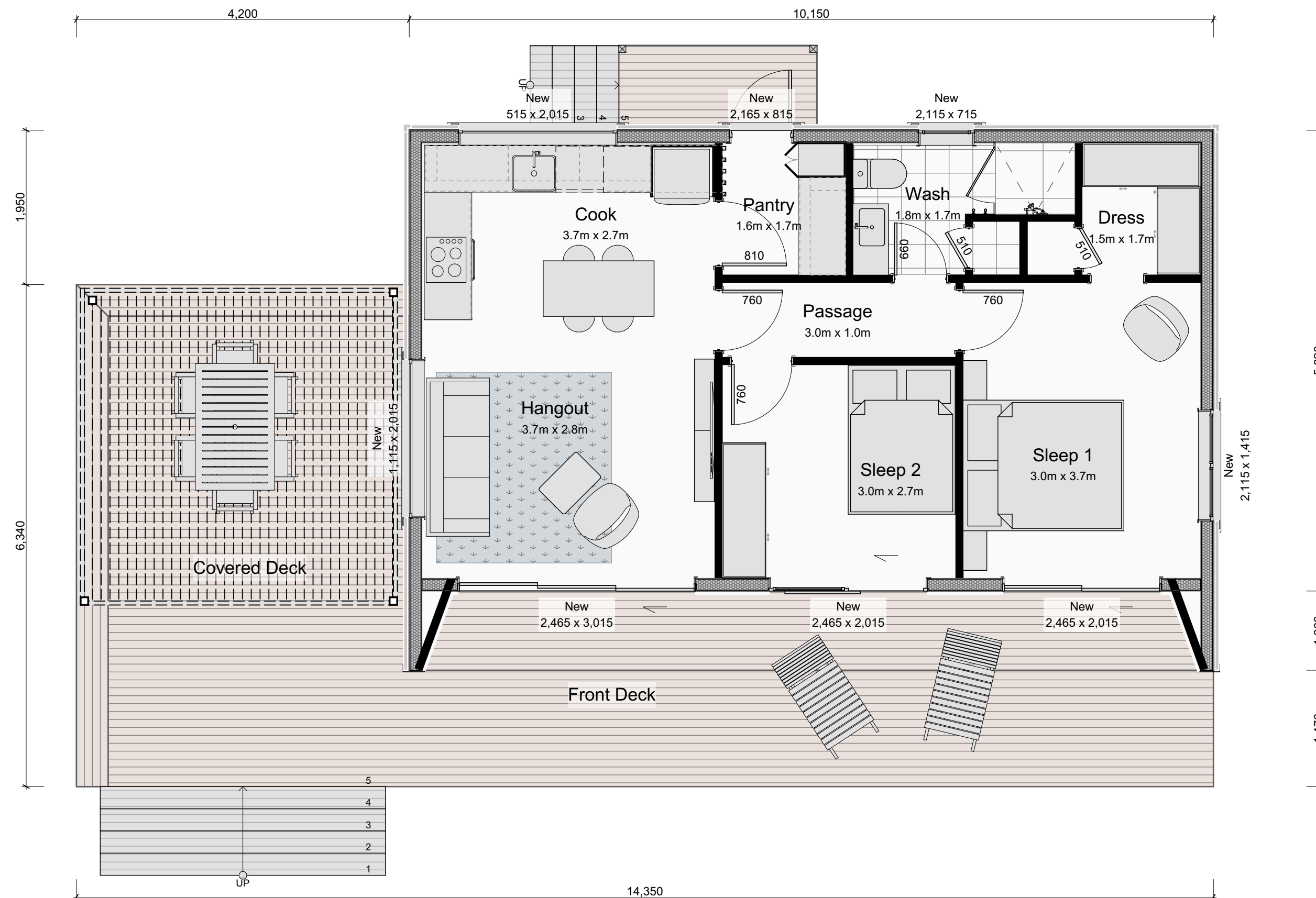
The Crib 60m2 scale 1:50
