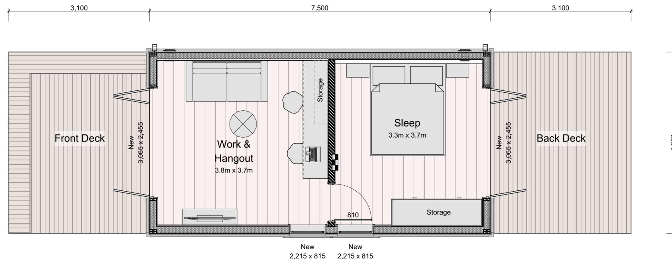
The Sleeper 30m2 scale 1:50
